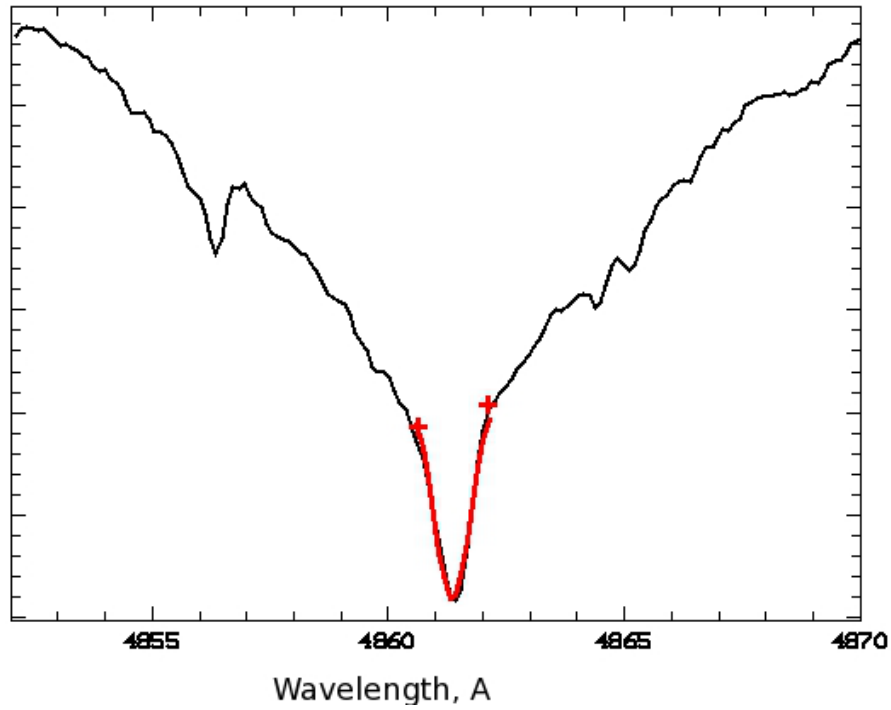
Figure 1: Hydrogen line core centre determination by fitting the line profile with a Gaussian
