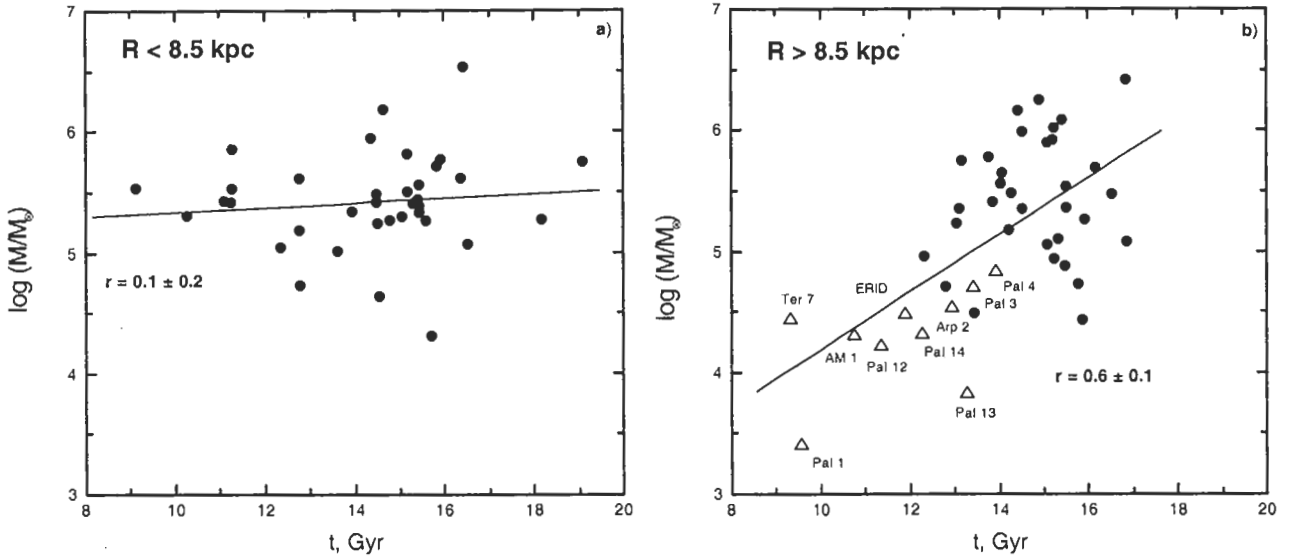
Figure 2: The mass-age relationship for the clusters lying inside (a) and outside (b) the solar circle. The straight lines are root-mean-square regressions, r are the corresponding correlation coefficients. The open triangles in diagram (b) show the clusters of anomalous mass the same as in Fig. 1b.
