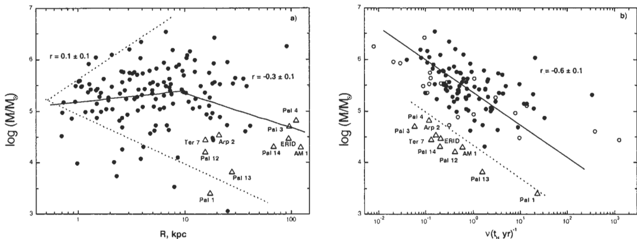
Figure 1: The relationship of the mass and the observed galactocentric distance R — (a), and that of the mass and the total dissipation velocity v taken from Gnedin, Ostriker (1997) — (b). The dotted line in diagram (a) shows the “cone of survival” according to the paper by Surdin and Arkhipova (1998). The thin lines are the straight lines of the regression in the regions inside and outside the solar orbit radius, while r are the corresponding correlation coefficients. The open triangles are for the clusters lying below the dotted line in diagram (b). The values of v in diagram (b) are expressed in units reverse to Hubble time adopted for convenience to be equal to 10 billion years. The open symbols (circles and triangles) denote the clusters lying farther than 15 kpc from the centre of the Galaxy. The solid line is a regression straight line for the main sequence of clusters, and the dotted line parallel to it separates the sequence of clusters of anomalously small mass shown by open triangles. Their names are beside them.
